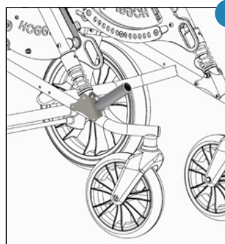
Preparation for mounting a “Buggypod”
