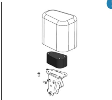
Abduction block 60 mm height extension kit
