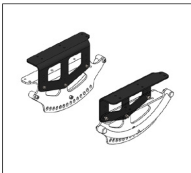
Seat height raiser, adjustable to 2, 4 or 6 cm
