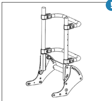
Universal-Back frame for seat shells
