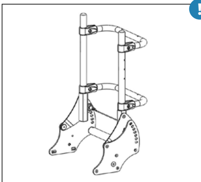
Universal-Back frame with physiological pivot point
