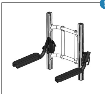
Armrests pivotably, angle adjustable with 270 mm PU Pads
