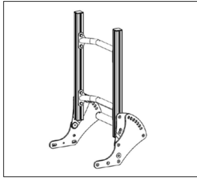
System-Profile-Back frame for seat shells
