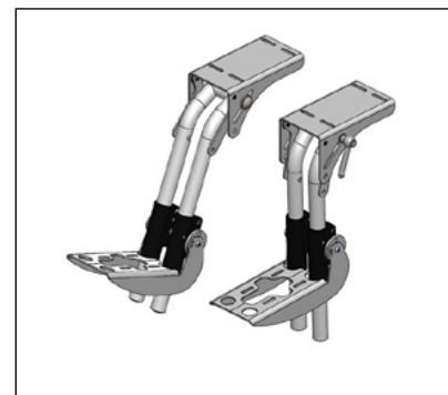
Single foot rest hanger, separat angle adjustable 85° - 160°
