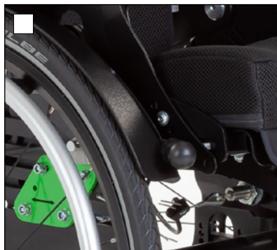
Integrated brake
