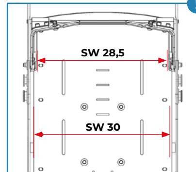
Top view // reduction of seat width by 1,5 cm
