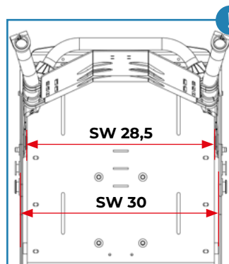
Top view // reduction of seat width by 1,5 cm
