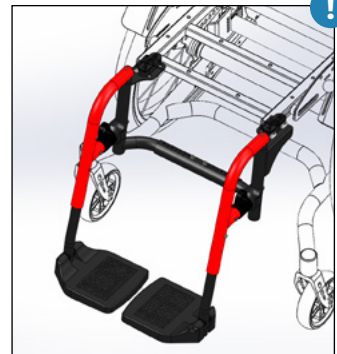
Adjustment to the SHERPA Vario Footrest system
