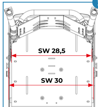
Top view // reduction of seat width by 1,5 cm
