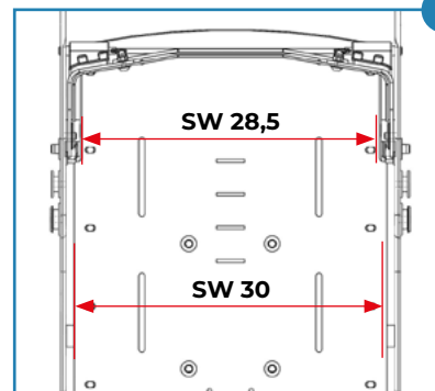
Top view // reduction of seat width by 1,5 cm
