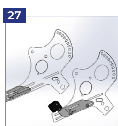
27 Retainer for accessories
