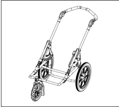
Cross with center steering wheel attachment
