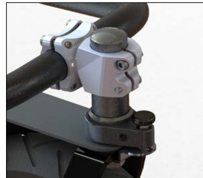
Swivellock for center steering wheel
