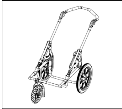
Cross with center steering wheel attachment, for additional devices
